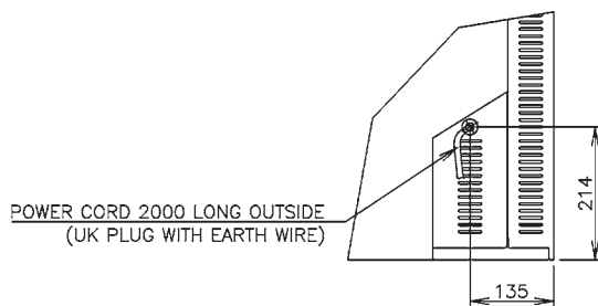
VIEW A(1/10)
